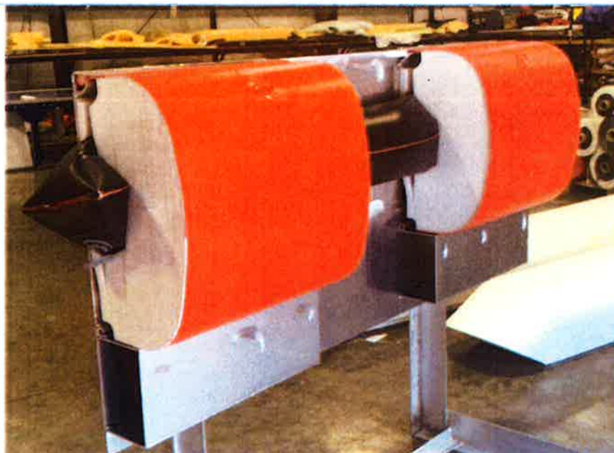
FIGURE 4: CUT-AWAY CROSS SECTIONS OF TYPICAL COLLAR
