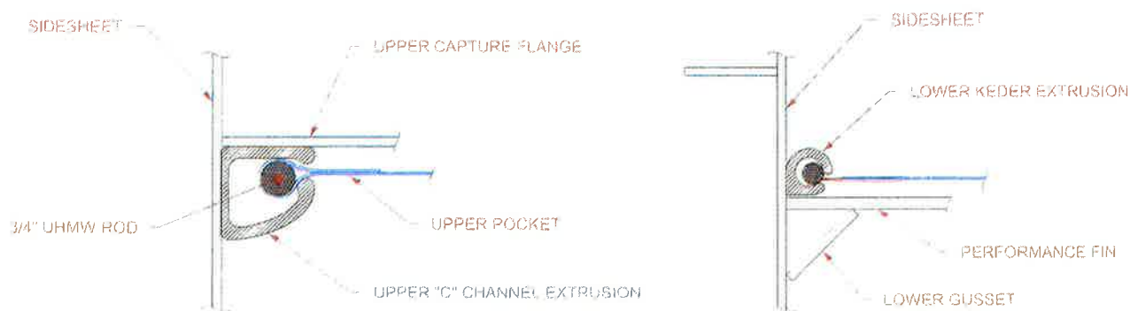
FIGURE 2 COLLAR ATTACHMENT EXTRUSIONS
