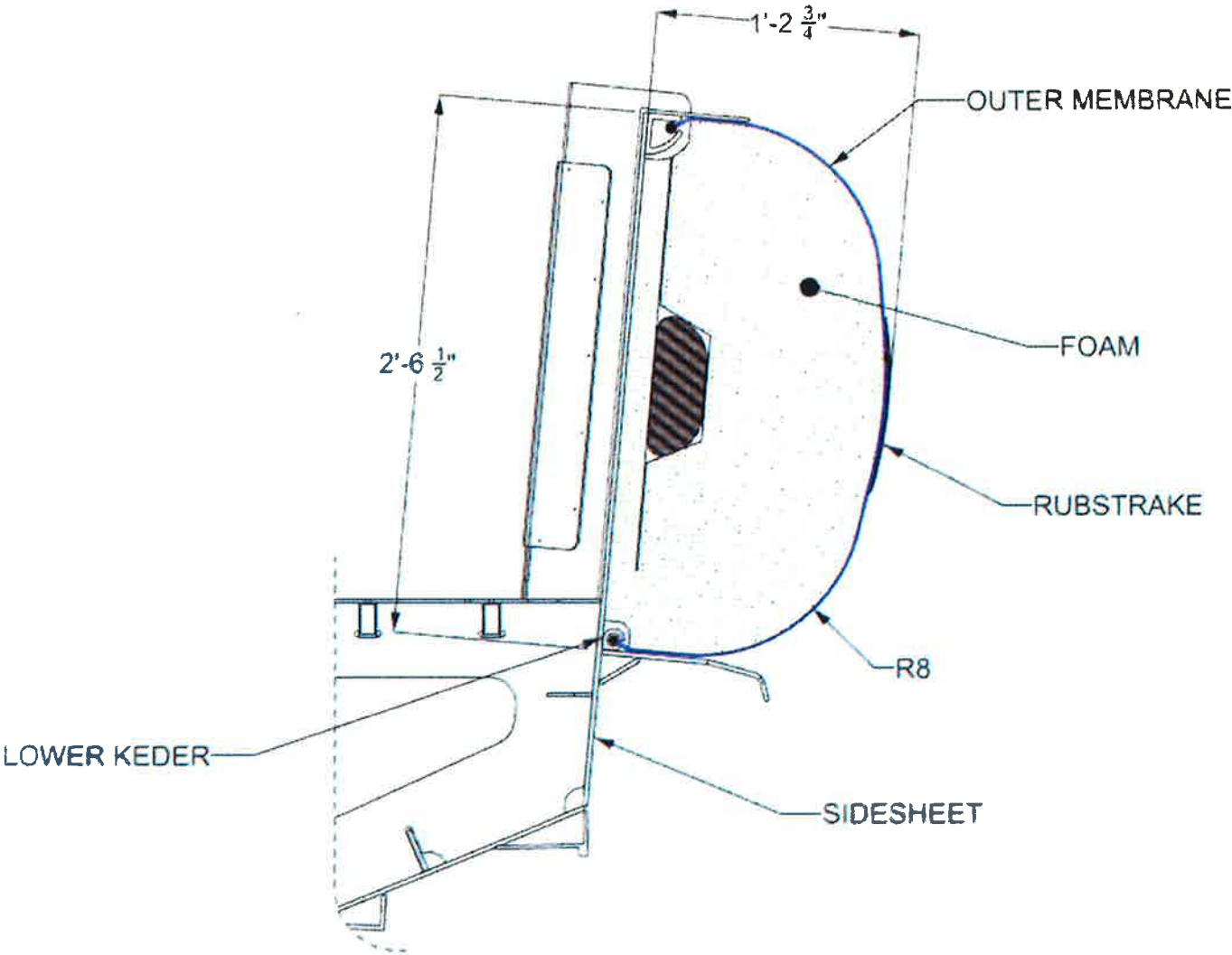
FIGURE 3: COLLAR CROSS-SECTION
