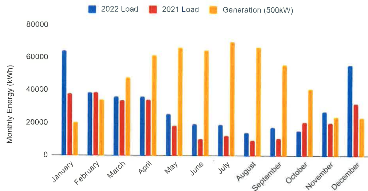
Normal Loads vs Generation
