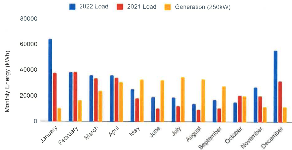
Normal Load vs Generation
